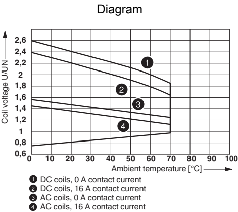
Operating voltage range
